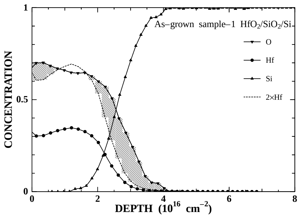
Fig. 3-2 The depth profiles of elements in the as-grown sample-1.
