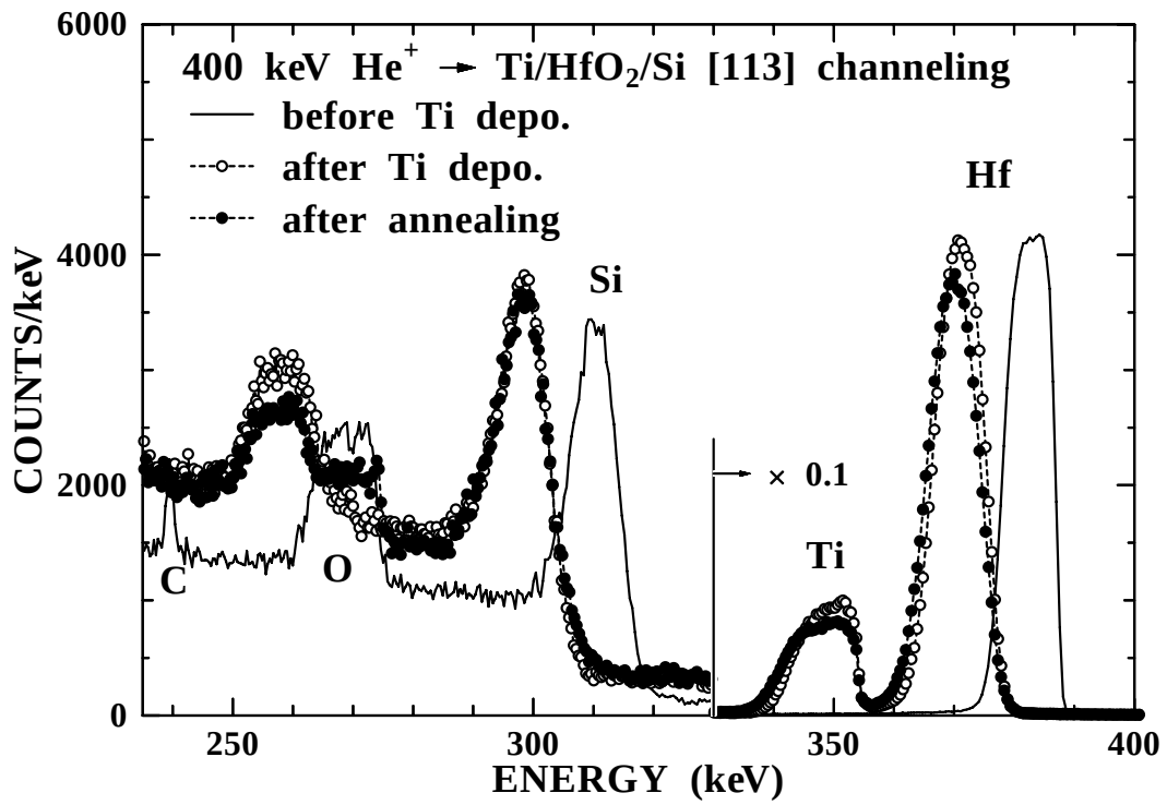
Fig. 5-1 HRBS energy spectra observed under [113] channeling conditions for the as-grown sample-2 \text{HfO}_2/\text{SiO}_2/\text{Si}(001) (solid line), after Ti deposition of 3.6 nm at RT (○) and after successive annealing at 330 °C for 30 min in UHV (●).
