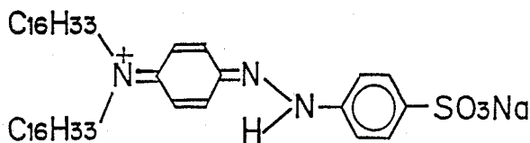
Hydrazone form
