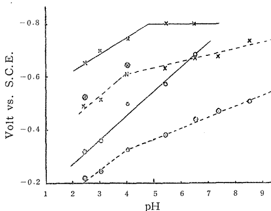
Fig. 1. Relation between deposition potential or half-wave potential and pH. ---x--- Bi on Pt; -⊗- Bi on Cu; ---○--- E_{1/2} -Bi; -○- Cu on Pt; ---○--- E_{1/2} -Cu.
