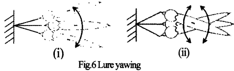
Fig.6 Lure yawing
