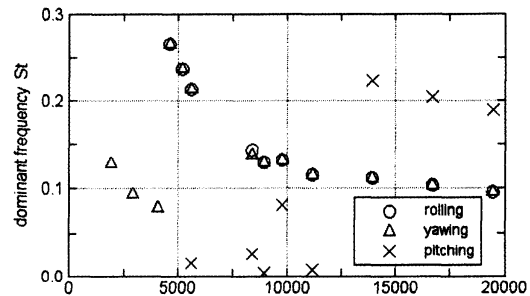
Fig.9 Reynolds number vs Strouhal number of the lure angles
