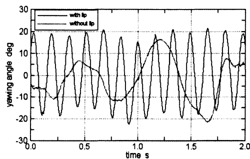
Fig.5 Time evolution of the yawing, Re=1.94 \times 10^4
