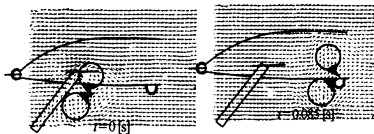
Fig.13 PIV results ( Re=1.11 \times 10^4 , side view)
