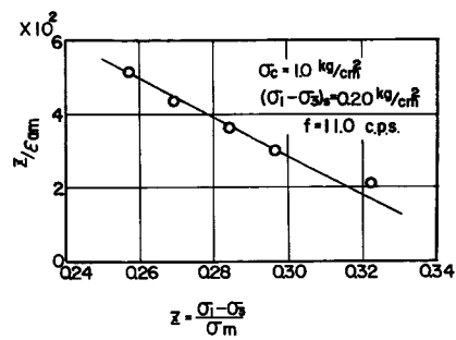
Fig. 7 Experimental relationship of Z/\varepsilon_{am} - Z constructed from Fig. 5.
