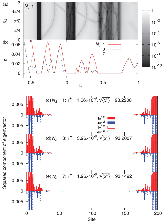
FIG. 7. (Color online) (a) Grayscale plots of \epsilon^+ for g = \sqrt{5} - 2 , \hat{B} = \hat{z} , L = 200 , (\Gamma, \alpha, V_Q) = (0.2, 0.3, 0.5) , \Delta = 0.1 , -0.6 \leq \mu \leq 1 , N_J = 1 , and 0 \leq \phi_J \leq \pi . (b) Value of \epsilon^+ plotted against \mu for N_J = 1, 3, 7 and \phi_J = \pi . Eigenstates for \mu = 0.04 are plotted for (c) N_J = 1 , (d) N_J = 3 , and (e) N_J = 7 .
