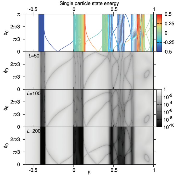
FIG. 6. (Color online) Top: Single particle eigenstates of Eq. (2) color coded according to the value of S_z for g = \sqrt{5} - 2 , \hat{\mathbf{B}} = \hat{z} , L = 200 , (\Gamma, \alpha, V_Q) = (0.3, 0.3, 0.5) , and 0 \leq \phi_0 \leq \pi . Lower: Grayscale plots of \epsilon^+ for the same set of parameters except that \Delta = 0.1 and -0.6 \leq \mu \leq 1 are introduced and L = 50, 100, 200 .
