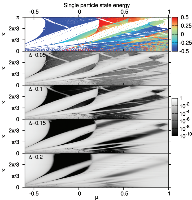
FIG. 4. (Color online) Top: Single particle eigenstates of Eq. (2) color coded according to the value of S_z for \hat{\mathbf{B}} = \hat{\mathbf{z}} , L = 400 , (\Gamma, \alpha, V_Q) = (0.3, 0.3, 0.5) , and 0 < \kappa < \pi . Lower: Grayscale plots of \epsilon^+ for the same parameters with \Delta = 0.05, 0.1, 0.15, 0.2 and -0.6 \leq \mu \leq 1 .
