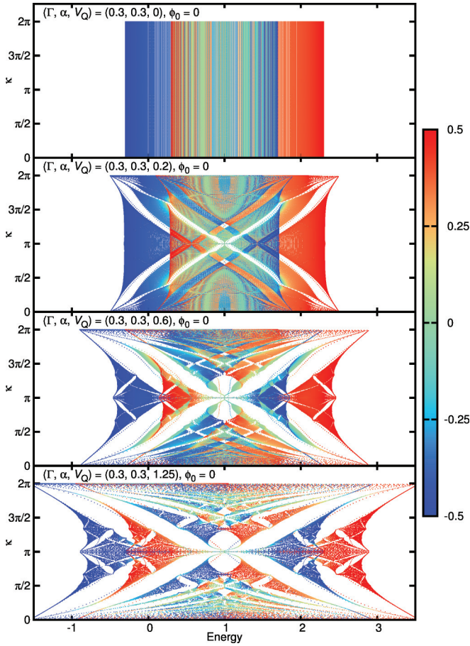
FIG. 1. (Color online) The distribution of single particle state energy of Eq. (2) for L = 200 , (\Gamma, \alpha) = (0.3, 0.3) , V_Q = 0, 0.2, 0.6, 1.25 , \hat{\mathbf{B}} = \hat{\mathbf{z}} . The single particle Hamiltonian (2) is diagonalized for \kappa = 2\pi j/400 ( j = 0, 1, \dots, 400 ) and each eigenstate is plotted in a color corresponding to the expectation value of the z component of the spin for that eigenstate. The plot for V_Q = 1.25 is similar to that for V_Q = 0.8 (not shown) except that the former is scaled horizontally, because of the duality of the lattice between V_Q = x and 1/x . V_Q = 1 is the self-similar point, at which the modulation potential equals the unmodulated bandwidth for \Gamma = \alpha = 0 .
