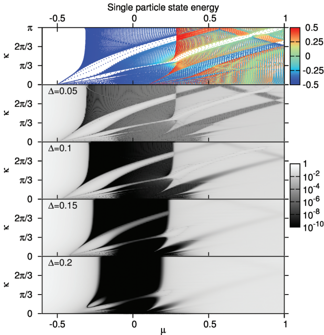
FIG. 3. (Color online) Top: Single particle eigenstates of Eq. (2) (nonsuperconducting case) color coded according to the value of S_z for \hat{\mathbf{B}} = \hat{\mathbf{z}} , L = 400 , (\Gamma, \alpha, V_Q) = (0.3, 0.3, 0.2) , and 0 < \kappa < \pi . Lower: Grayscale plots of \epsilon^+ for the same parameters with \Delta = 0.05, 0.1, 0.15, 0.2 and -0.6 \leq \mu \leq 1 .
