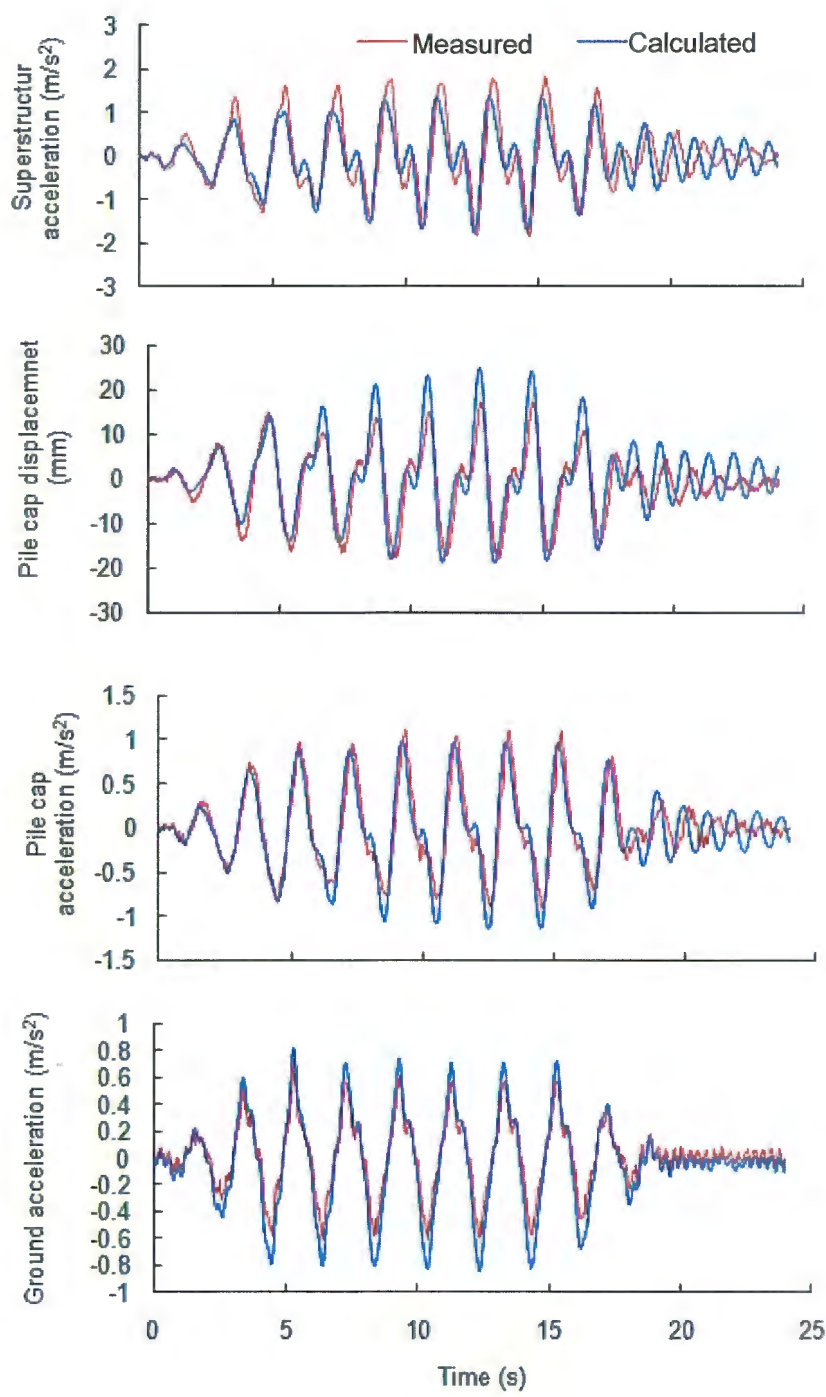
Fig. 7.11 Comparison of recorded and calculated ground and pile cap responses, with superstructure, 0.5 Hz
