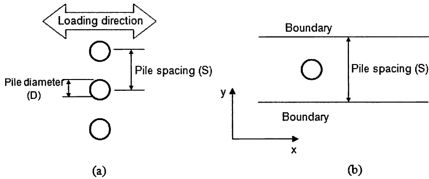
Fig. 3.7 Soil-pile system in horizontal plane: (a) single row of equally spaced pile group (plane view); (b) analysis domain for a single pile in the group
