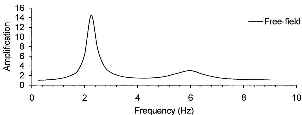
Fig. 9.2 Free-field response
