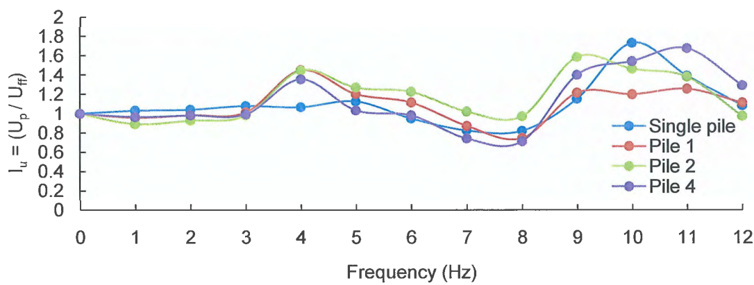
Fig. 8.17 Kinematic interaction factors of piles versus base excitation frequencies
