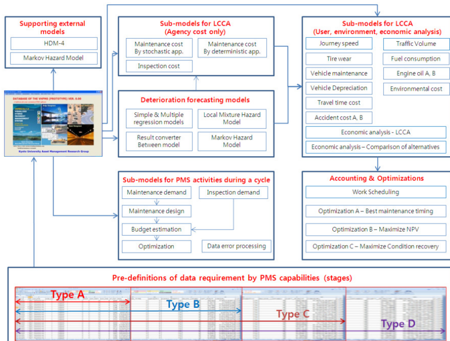
Figure 2.3 Suggestion of a general framework of PMS (full version)
