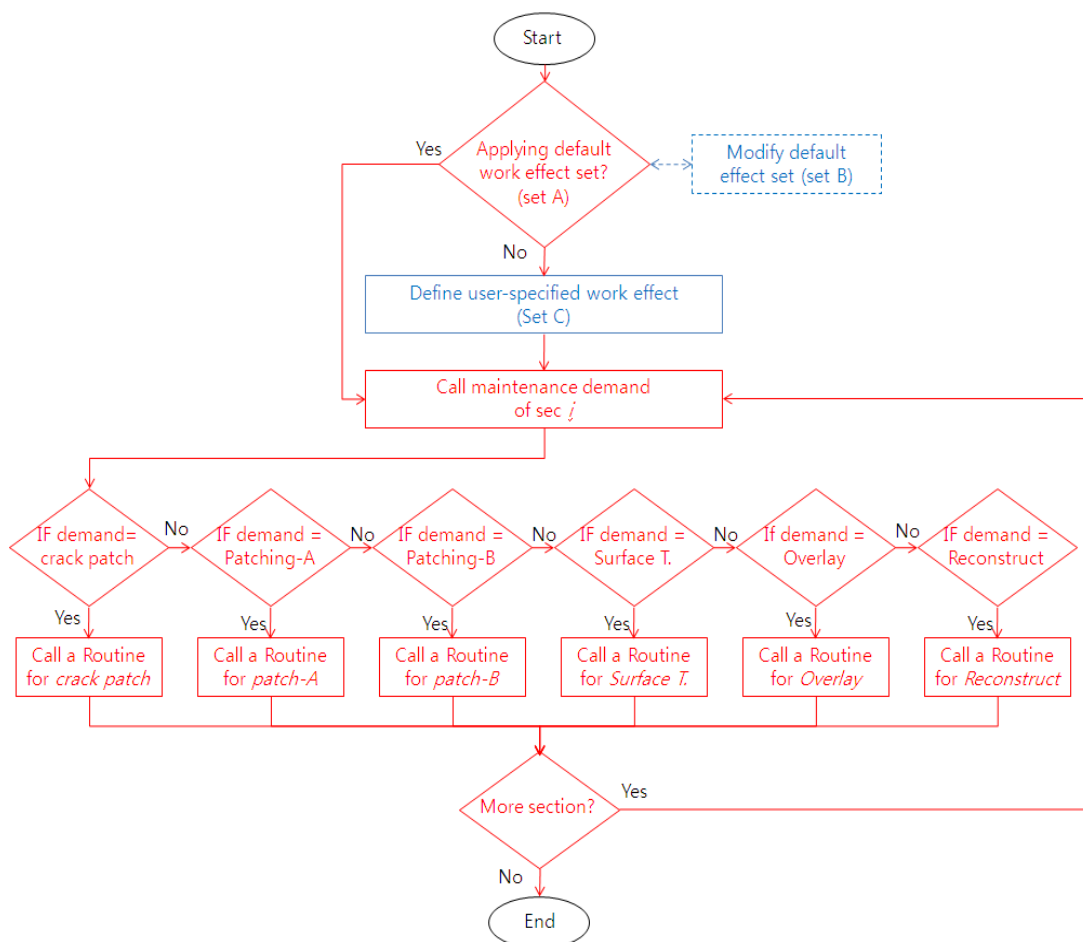
Figure 4.3 A flowchart for maintenance effect model
