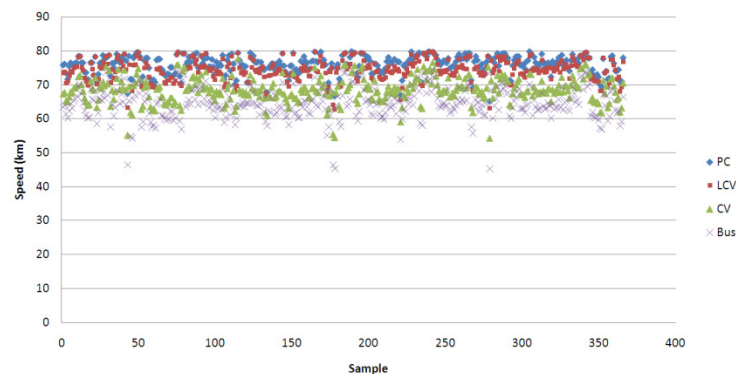
Figure 6.24 Estimated journey speeds (case: 4 lanes, 80km speed limit, and enforcement factor 1.0)
