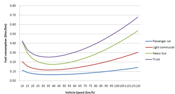
Figure 6.7a Fuel consumption model of Hybrid PMS (left)
