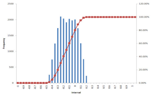
Figure 6.29d A case for a decreasing trend (Case: \varepsilon_l^{TC}=0.2 , \varepsilon_l^{DC}=0.5 )
