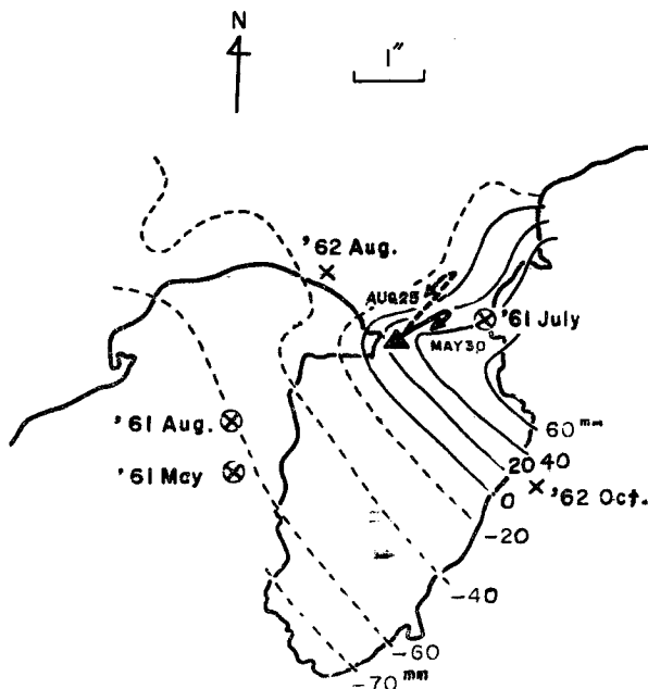
Fig. 11 Vertical movements in the period from 1925 to 1931 (after Dambara) and vector diagram of anomalous ground tilts for two groups of earthquakes.
