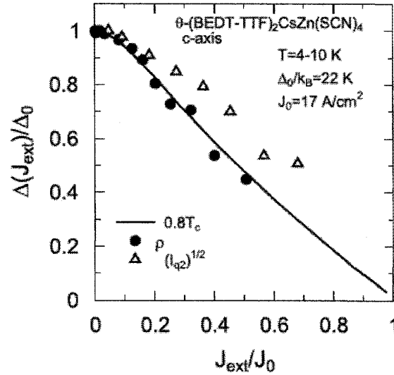
Figure 3: The comparison the experiment done by my group and with the calculation by Ajisaka and Tasaki. The solid curve is the calculation with a reasonable value of T/T_c=0.8 . The circles and triangles are the experimental data from the resistivity and the x-ray diffraction, respectively. The experimental data are properly normalized with the parameters of a critical current J_0 and an energy gap \Delta/k_B at 0 K, which are written in the right upper part of the figure.
