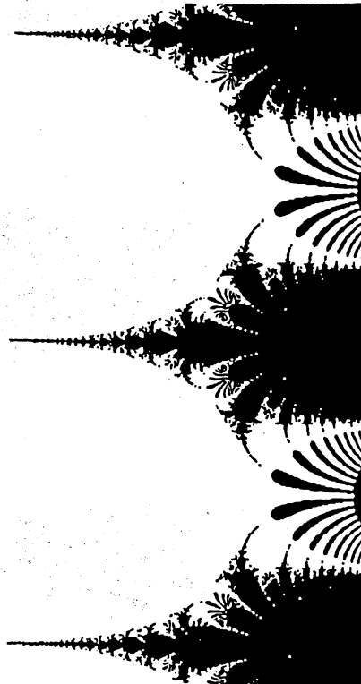
Figure 5: \log \lambda = 0
