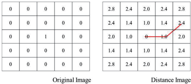
図 17 Distance transeform.
