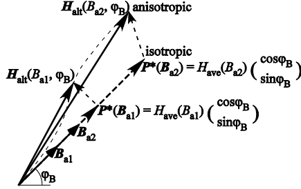
Fig. 3. Relation between H_{\text{ave}}(\mathbf{B}) and \mathbf{H}_{\text{alt}}(\mathbf{B}, \varphi_B) .
