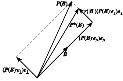
Fig. 2. Relation between \mathbf{P} and \mathbf{P}^* .
