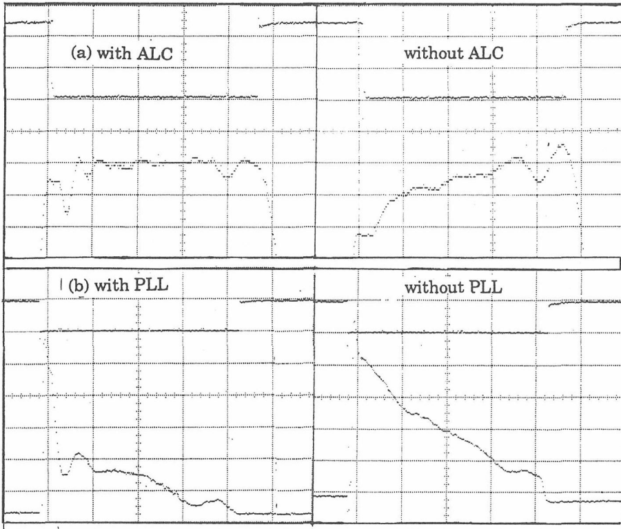
Figure 8 (a) The RF amplitude error with ALC and without ALC in the RFQ cavity (0.5%/div).
