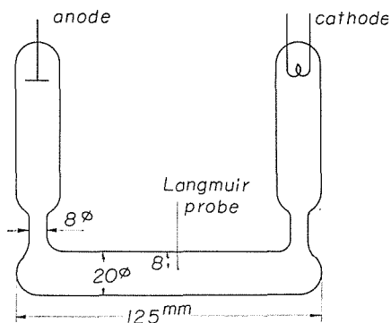
Fig. 3. Discharge tube.
