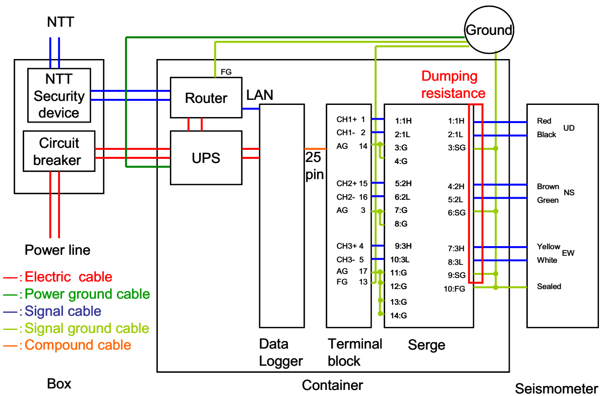
b. Connection for the online system
