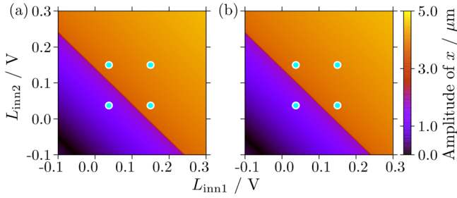
FIG. 4. Amplitude modulation systematically varied in input signals L_{inn1} and L_{inn2} at f_n = 8.6654 kHz and V_{dcn} = 150 mV (numerical results). The light (dark) region corresponds to more than (less than) 3.0 \mu\text{m} in displacement amplitude, corresponding to a logical “1” (logical “0”) output. For an OR gate, input signals are set to 150.0 mV and 37.5 mV, as shown by the four circles with light (aqua) color: (a) Initial state is set to the large amplitude solution (logical “1” for memory output) (b) Initial state is the small amplitude solution (logical “0” for memory output).
