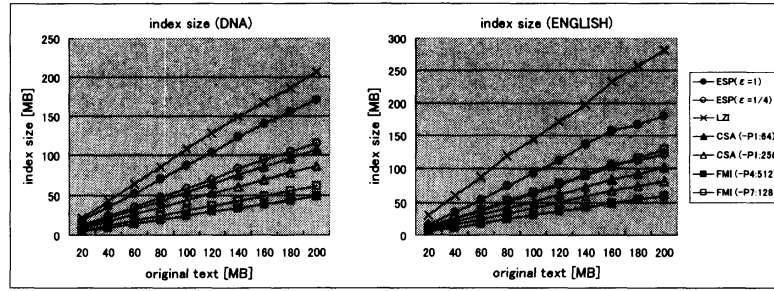
Figure 8: Index Size.
