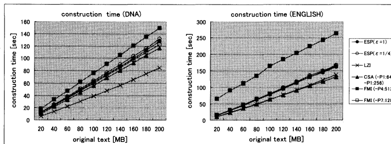
Figure 7: Construction Time.
