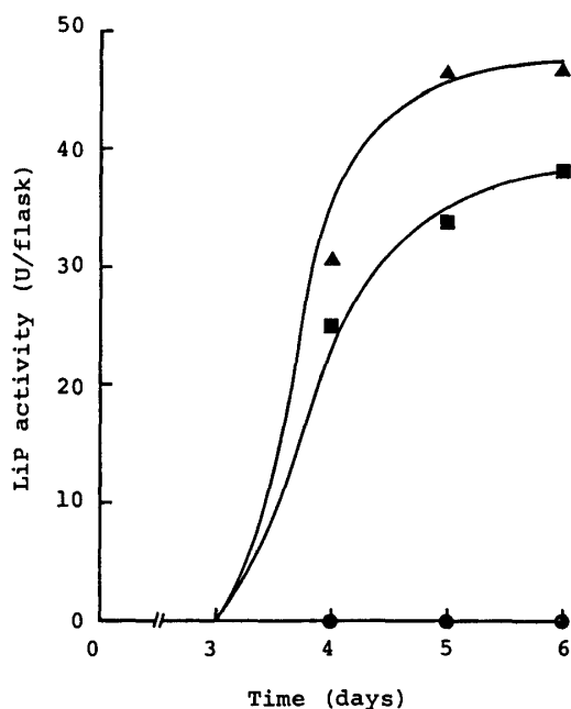
Fig. 4. Effects of MnSO_4 and MnO_2 on LiP production by P. chrysosporium under the shaking culture conditions (6 PU cubes/flask, at 200 rpm for the first 60 hr and then at 125 rpm).
