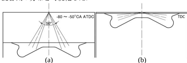
Fig. 1. Spray layout
