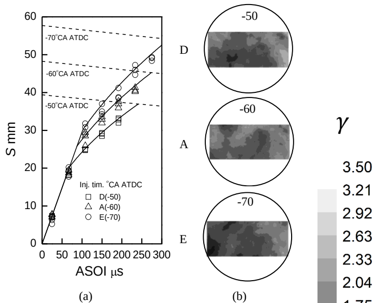
Fig. 6. Effects of injection timing on liquid penetration (a) and fuel distribution at TDC (b).
