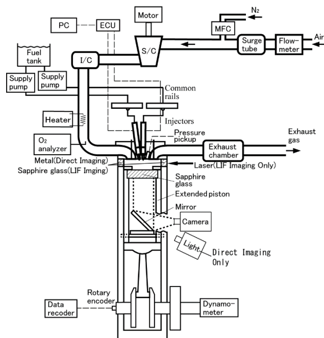
Fig. 2. Experimental setup
