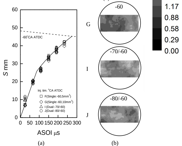
Fig. 8. Effects of multi-stage injection on liquid penetration (a) and fuel distribution at TDC (b).
