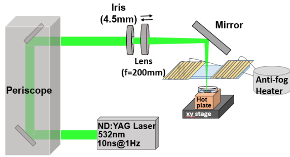
Fig. 1. Experimental setup.
