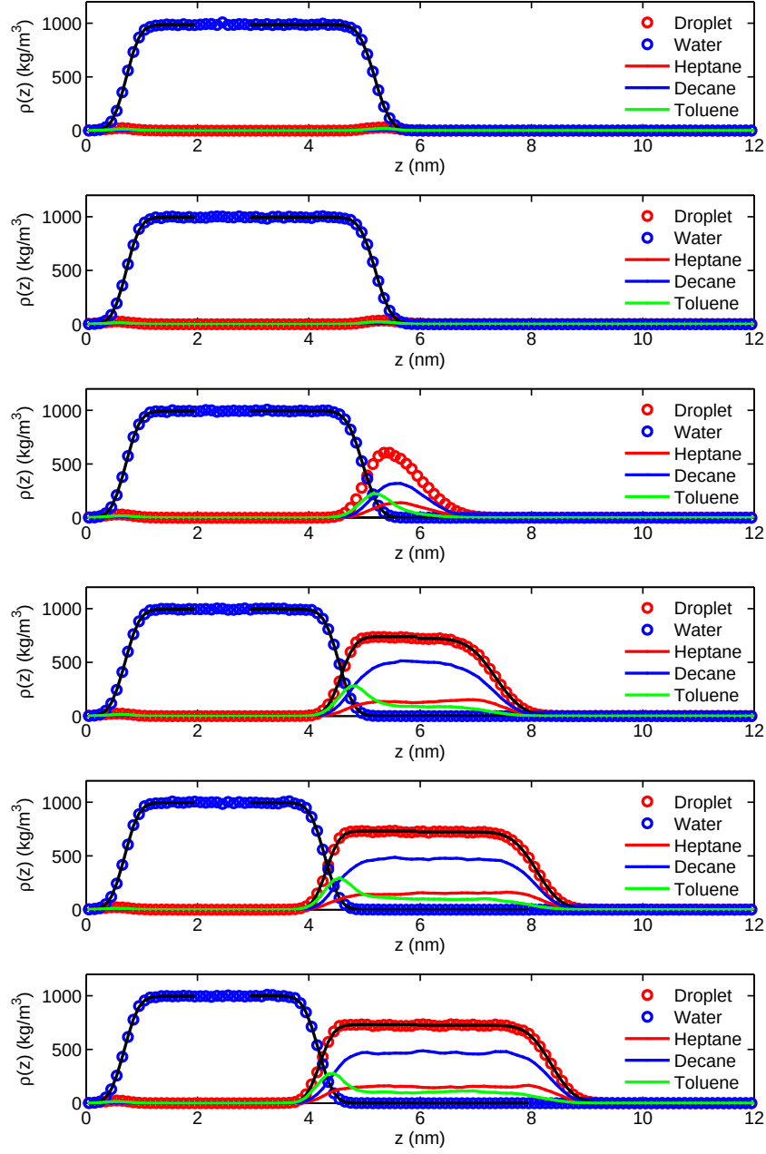
Figure 5.7: Density profiles for multicomponent-oil-water-vapor three phase system along z -axis at x=0, 2, 4, 6, 8 and 10\text{nm} (from top to bottom). The density profile of droplet was calculated as the summation of the densities of heptane, decane and toluene. Solid lines show fitted curves for the density profiles of water and droplet.
