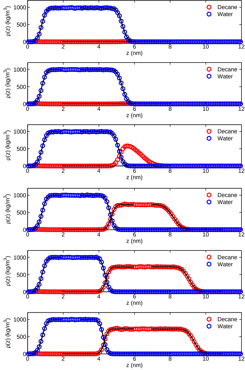
Figure 4.18: Density profiles for decane–water–vapor three phase system along z -axis at x=0, 2, 4, 6, 8 and 10 nm (from top to bottom). Solid lines show fitted curves for the density profiles of water and decane.
