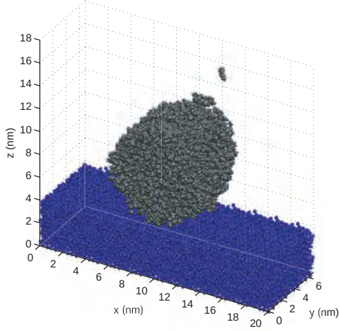
(c) 3D view at 0 ns
