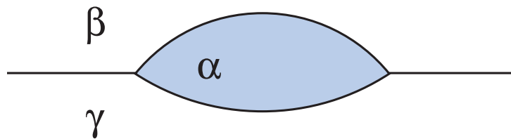
Figure 4.2: Coexistence of three fluid phases.
