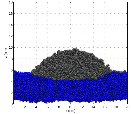
(b) side view at 5 ns
