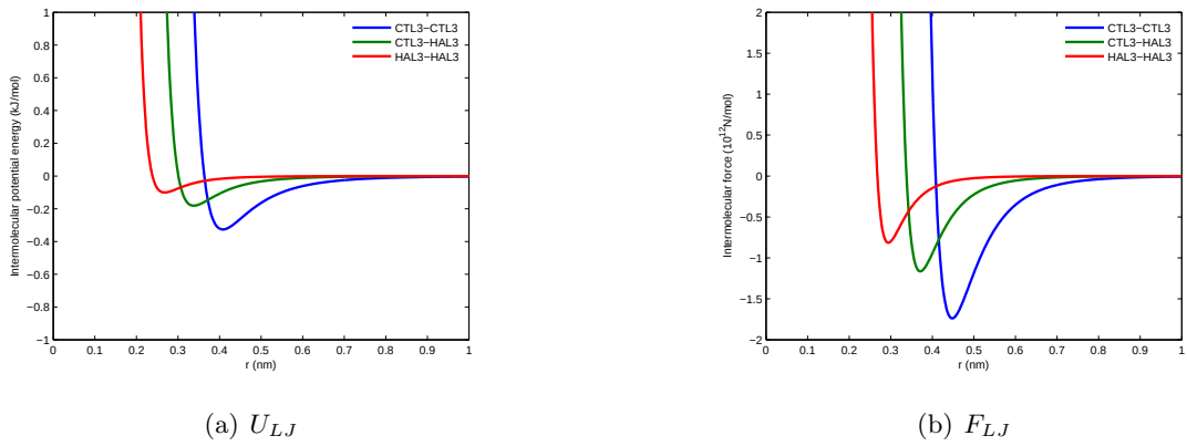
Figure 2.2: Comparison of U_{LJ} and F_{LJ} between CTL3-CTL3, CTL3-HAL3 and HAL3-HAL3.
