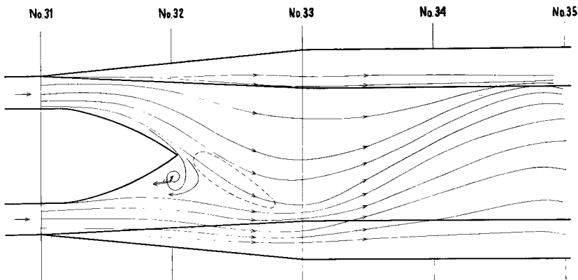
Fig. 29 Hydraulic behavior for the abrupt expansion (The type of transition is A)
