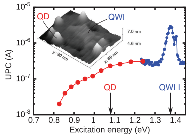
FIG. 2. (Color online) UPC excitation spectrum for sample C. The two main features are photocurrent due to excitation of the QWIs and QDs. The indicated energy levels of the shallowest QWI I and the QDs were determined from PL. Inset: 3D AFM image with QDs and a QWI on the WL of an InAs/AlGaAs layer without capping.
