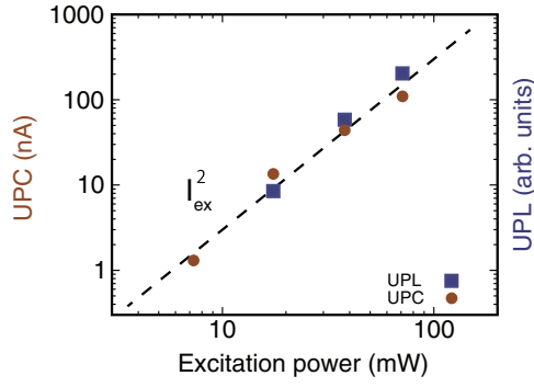
FIG. 8. (Color online) Power dependence of UPL and UPC for excitation of QWI I at 20 K. Both UPL and UPC trends indicate that a nonlinear process is responsible for the efficient upconversion in shallow QWIs. For a guide to the eye we plotted the broken line I_{ex}^2 , representing a quadratic power dependence on the excitation intensity.
