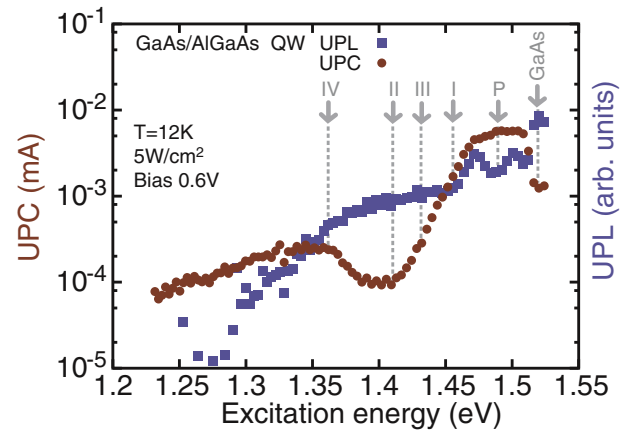
FIG. 7. (Color online) Comparison of UPL and UPC. P indicates the phonon-assisted upconversion peak. I, II, and III mark the peak positions of the shallow QWIs.
