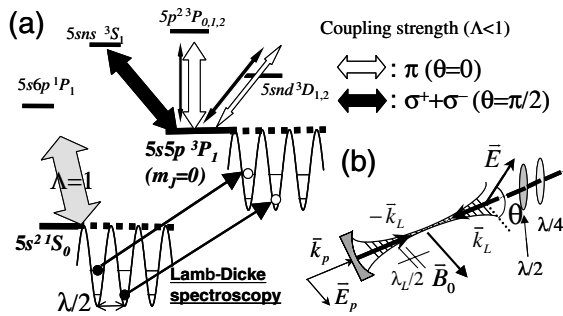
FIG. 1. (a) Level diagram and optical coupling related to the {}^1S_0 - {}^3P_1 clock transition. The {}^1S_0 state is dominantly coupled to {}^1P_1 , while the {}^3P_1 state is coupled to the upper triplet states of {}^3S , {}^3P , and {}^3D . The latter couplings strongly depend on the light polarization, as depicted by the thickness of arrows. (b) Schematic diagram of the 1D optical lattice. A bias magnetic field \vec{B}_0 was applied parallel to the probe electric field \vec{E}_p with a wave vector \vec{k}_p parallel to that of the lattice beam \pm \vec{k}_L . \theta represents an angle between \vec{B}_0 and the electric field \vec{E} of the lattice. The probe laser was introduced parallel to \pm \vec{k}_L , along which the spatial modulation of the ac Stark shift confines atoms in the LDR, as depicted in (a).
