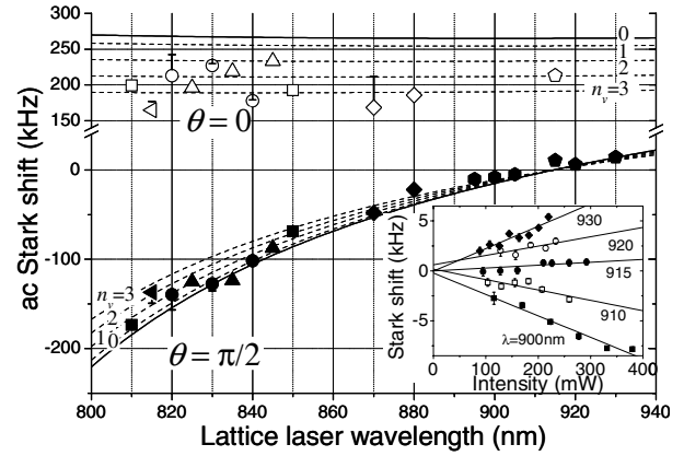
FIG. 3. Differential Stark shift for the ^1S_0 - ^3P_1(m = 0) transition. The shift depends on the trap laser wavelength \lambda_L , the polarization rotation \theta , and the vibrational state n_v , indicated by dashed lines. Different symbols correspond to the measurements on different days. The inset shows the intensity dependence of the shifts measured for several wavelengths \lambda_L at \theta = \pi/2 . By linearly extrapolating to zero laser power, the atomic resonance frequency was obtained.
