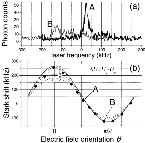
FIG. 2. (a) Fluorescence spectra of Sr atoms confined in a 1D optical lattice for different polarization orientation \theta at \lambda_L = 830 nm. At \theta \approx \pi/4 (A), the narrower spectrum was observed as the Stark shifts on the clock transition nearly canceled out, whereas nonzero differential Stark shift introduced a frequency shift and broadening for \theta \approx \pi/2 (B). (b) The change of the Stark shift as the angular orientation \theta of the lattice-laser polarization with respect to a bias magnetic field. Since the light shift of the ^3P_1(m_J = 0) depends on the lattice laser polarization, the frequency varies sinusoidally depending on the components of \pi and the \sigma^+ + \sigma^- intensity. The dashed lines show the differential Stark shifts for atoms in the n_v = 0, 1, 2 vibrational states.
