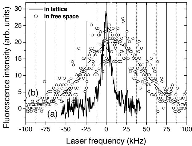
FIG. 4. Laser-induced fluorescence of atoms (a) confined in a 1D optical lattice and (b) in free fall. The dashed line shows a Gaussian fit to the data points (b). The confinement suppressed the Doppler width of 83 kHz and gave a narrow Lorentzian linewidth of 11 kHz, which was limited by the saturation broadening. A slight blueshift of the center frequency in (b) is caused by the photon recoil shift.
