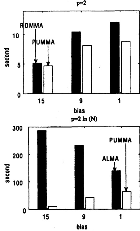
Figure 4: Computation time over artificial data set in the case p = 2 (upper) and p = 2 \ln(n) (lower).
