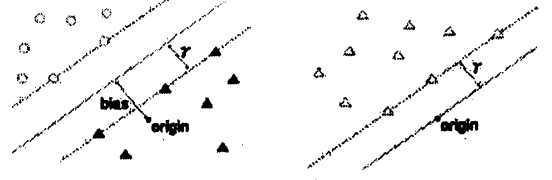
Figure 2: Illustration of the implicit reduction which preserves the margin.
