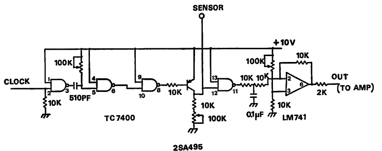
(a) Circuit 1
