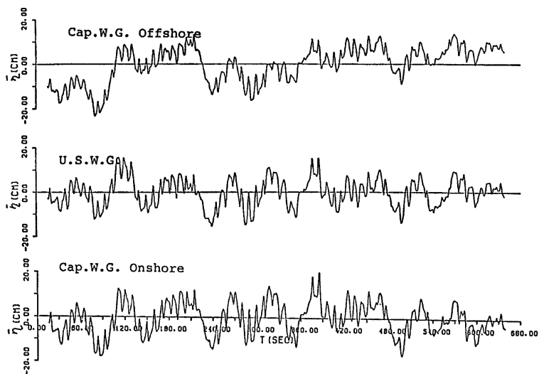
Fig. 17 Comparison of average sea level measured with capacitance- and sonic-type wave gauges
