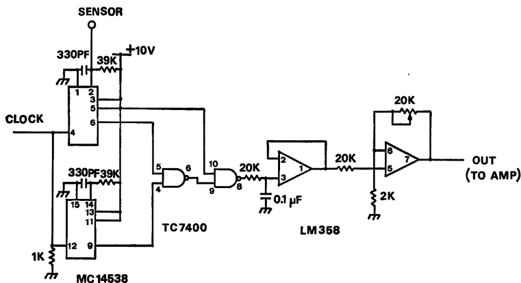
(b) Circuit 2
