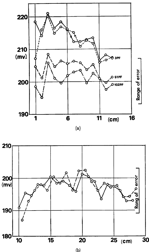
Fig. 8 Results of calibration of capacitance-type wave gauge of teflon wire
