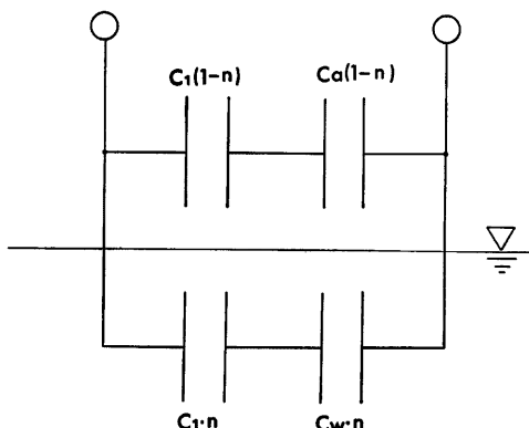
Fig. 2 Schema of capacitance connected in water showing principle capacitance-type wave gauge
