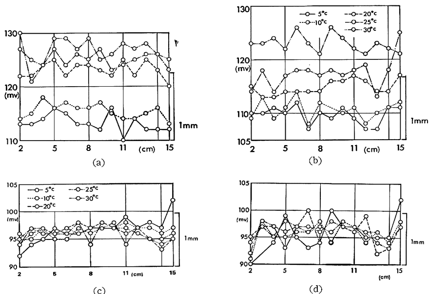
Fig. 5 Results of calibration of capacitance-type wave gauges
