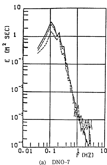
Fig. 16 Spectral properties of waves measured with capacitance- and sonic-type wave gauges
