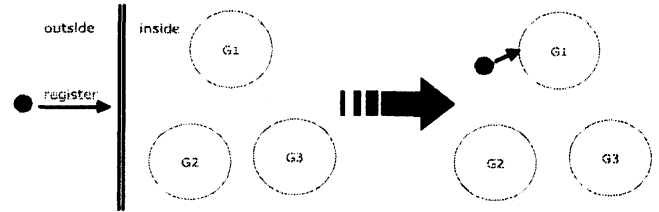
Figure 2. Initialization process. If a peer wants to join the system, it should register firstly. And the system will assign a unique identity to him, and then map the peer into a group (In the example, G_1 chosen) based on certain principle.
