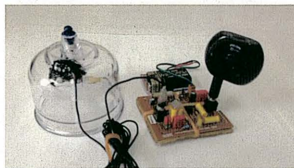
Fig. 3: Prototype suction cup connected to a home-made amplifier and its external battery providing fetal cardiac signal to HP8041A via Bluetooth transceiver.
