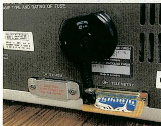
Fig. 4: Bluetooth receiver connected to the telemetry port of HP8041A
