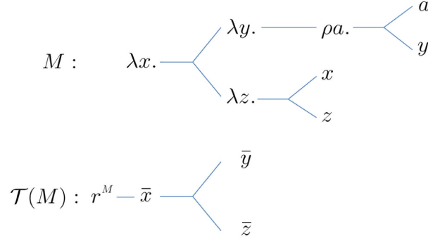
FIGURE 1. M \equiv \lambda x.(\lambda y.\rho a.ay)(\lambda z.xz)
