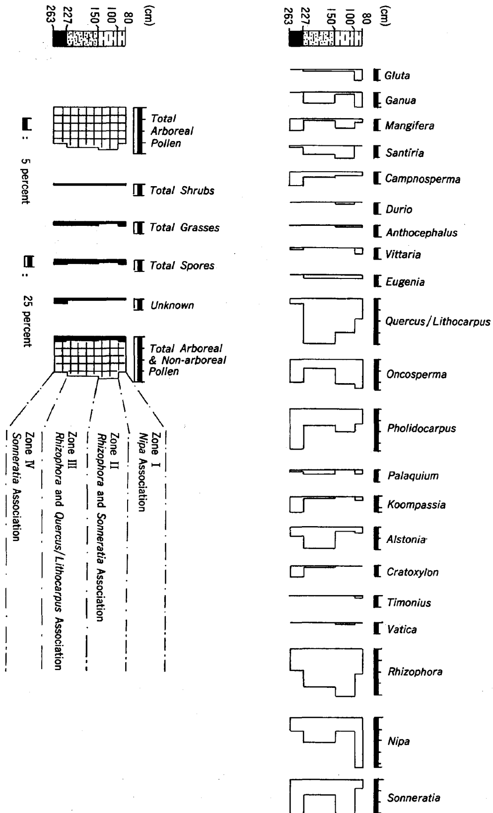
Fig. 6a The Pollen Diagram of Profile T-24
