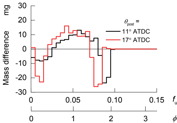
Figure 23 Mass-difference against the mixture fraction f_u at 5° ASl post (10-hole nozzle, p_i = 130 MPa).
