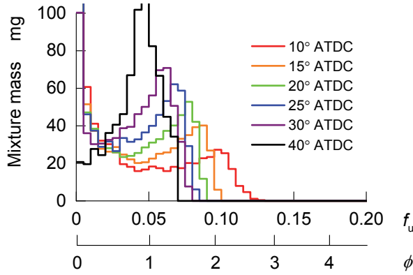
Figure 22 Histograms for the mixture fraction f_u (10-hole nozzle, without post injection, main-injection quantity: 27 mm 3 , p_i = 130 MPa).
