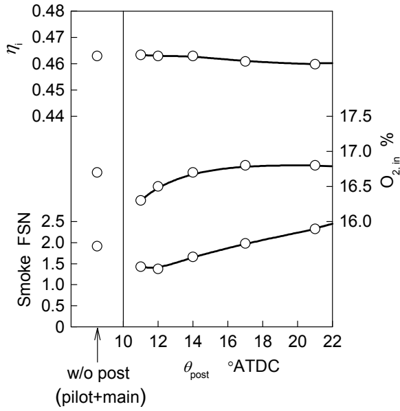
Figure 2 Effects of the post-injection timing on the indicated thermal efficiency \eta_i , intake oxygen concentration O_{2,\text{in}} , and smoke emission (experimental results).
