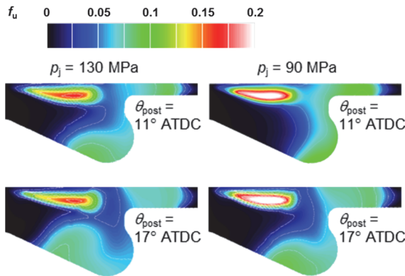
Figure 24 Distributions of the mixture fraction f_u at 3° ASl post (10-hole nozzle, p_i = 130 MPa and 90 MPa, \theta_{post} = 11° and 17° ATDC).
