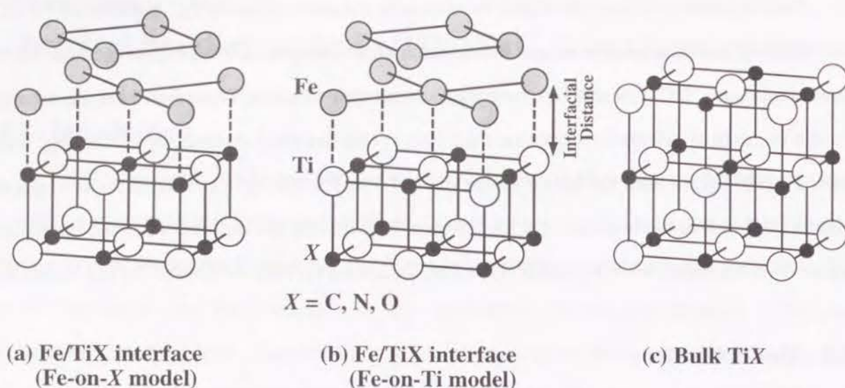
Fig. 6-2 The structure of model clusters employed in this work ( X = \text{C, N or O} ). (a) \text{Fe}_9\text{-Ti}_9\text{X}_9 cluster for the Fe/TiX interfaces where the Fe atoms are on X atoms. (b) \text{Fe}_9\text{-Ti}_9\text{X}_9 cluster for the Fe/TiX interfaces where the Fe atoms are on Ti atoms. (c) \text{Ti}_{14}\text{X}_{13} cluster for bulk TiX.
