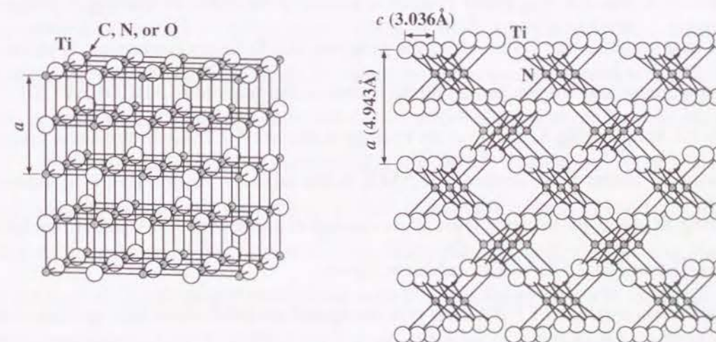
(a) TiX (X=C, N or O) (b) Ti 2 N
