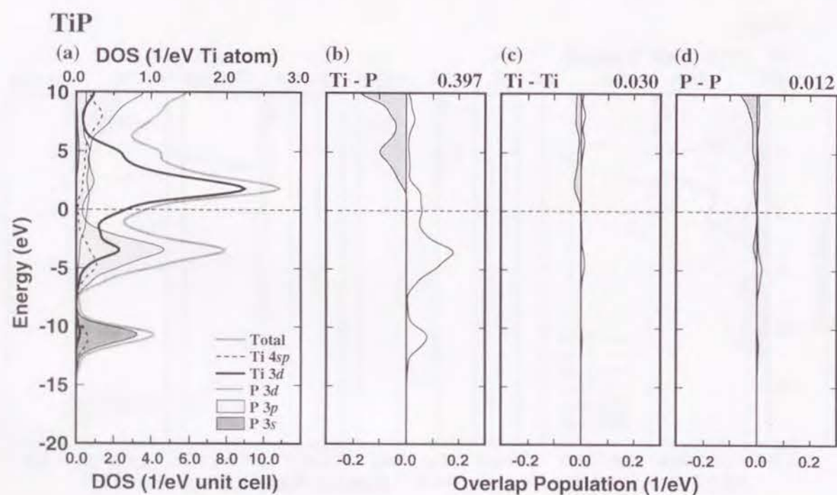
Fig. 3-24 Total and partial density of states and the overlap population diagrams for \text{TiP} . (a) Total and partial density of states (b) overlap population diagram for the Ti-P bond (c) for the Ti-Ti bond (d) for the P-P bond.
