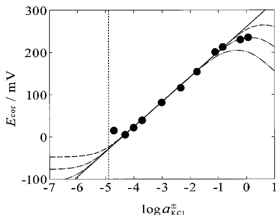
Fig. 3 Plots of E_{\text{cor}} against \log a_{\text{KCl}}^{\pm} for the KCl aqueous solution-[TOMA + ][C 4 C 4 N - ] (containing DCH18C6 and K + [C 4 C 4 N - ]) two-phase system represented as cell (B) at various concentrations of KCl in an aqueous solution. The solid line represents a line with the Nernstian slope at 25°C (59.2 mV/decade). Three curves are from a calculation of the phase-boundary potential with K_{\text{ML}} = 1 \times 10^8 (dashed line) 1 \times 10^9 (dashed dotted line), and 1 \times 10^{10} (dashed double-dotted line) and other fixed parameters (see Table 2). The vertical dotted line shows the solubility of AgCl in water ( 13 \mu\text{mol dm}^{-3} ).
