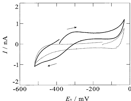
Fig. 1 Cyclic voltammograms for the ion transfer across the interface between a 10 mM KCl aqueous solution and [TOMA + ][C 4 C 4 N - ] in the presence (solid line) and the absence (dotted line) of 20 mmol kg -1 DCH18C6 in [TOMA + ][C 4 C 4 N - ]. Scan rate, 10 mV s -1 ; inner diameter of the micropipette tip, 28 \mu\text{m} .
