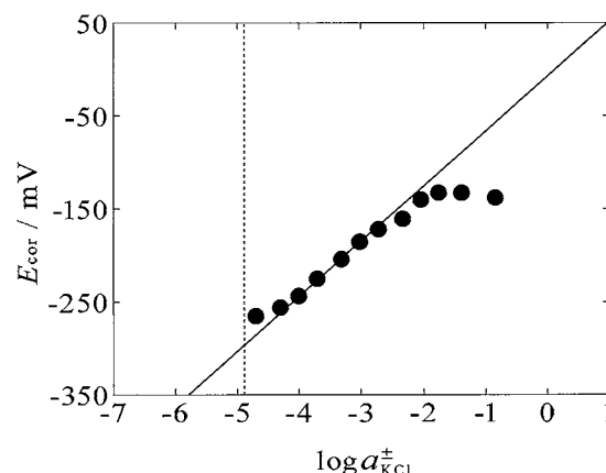
Fig. 4 Plots of E_{\text{cor}} against \log a_{\text{KCl}}^{\pm} for the KCl aqueous solution-gelled [TOMA + ][C 4 C 4 N - ] (containing DCH18C6 and K + [C 4 C 4 N - ]) two-phase system represented as cell (C) at various concentrations of KCl in the aqueous solution. The solid line represents a line with the Nernstian slope at 25°C (59.2 mV/decade). The vertical dotted line shows the solubility of AgCl in water ( 13 \mu\text{mol dm}^{-3} ).
