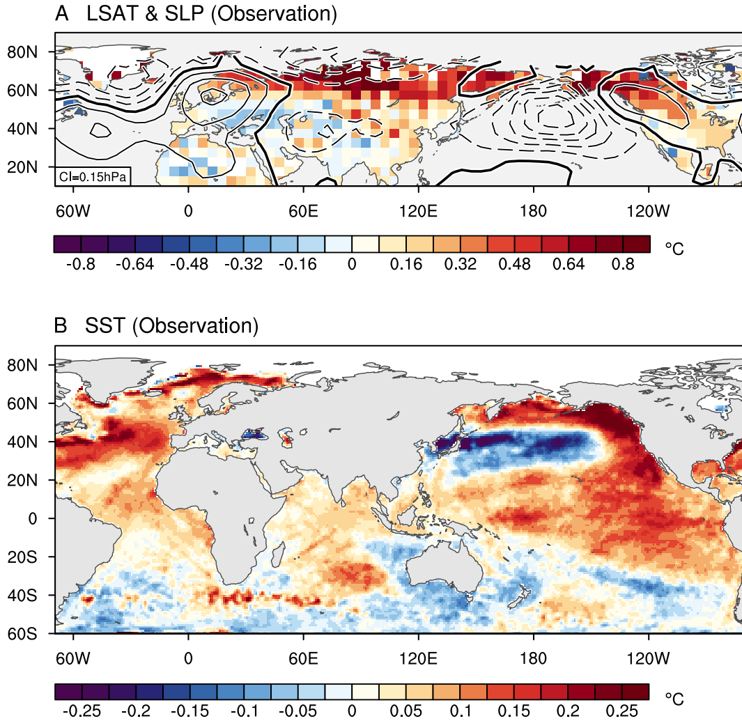
Fig. S8. Observed anomalies of (A) LSAT and SLP, and (B) SST regressed onto the normalized Arctic mean LSAT anomaly for 1900-2000. LSAT, SLP, and SST are obtained from the Climatic Research Unit Temperature version 4.4 (CRUTEM4.4), ICOADS/ISPD, and HadISST2, respectively. Detrended, 8-year low-pass filtered November-March mean anomalies are used.
