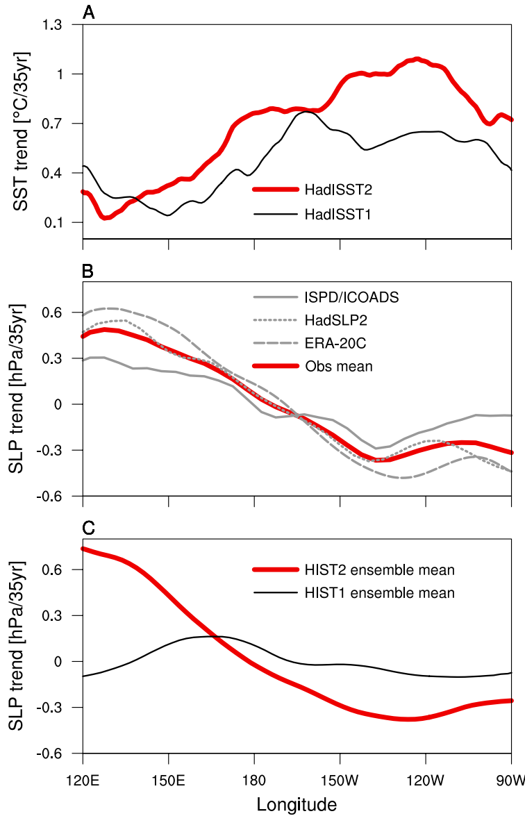
Fig. S3. Comparison of November-March mean SST and sea level pressure (SLP) trends averaged over the tropical Pacific (10°S-10°N) for 1908-1942. (A) SST trends from HadISST2 (red) and HadISST1 (black), (B) observed SLP trends from the International Surface Pressure Databank/International Comprehensive Ocean-Atmosphere Data Set (ISPD/ICOADS; gray solid), the UK Met Office Hadley Centre mean SLP (HadSLP2; gray short dashed), the European Centre for Medium-range Weather Forecast 20th-Century Reanalysis (ERA-20C; gray long dashed) and their mean (red), and (C) simulated SLP trends from the HIST2 (red) and HIST1 (black) experiments.
