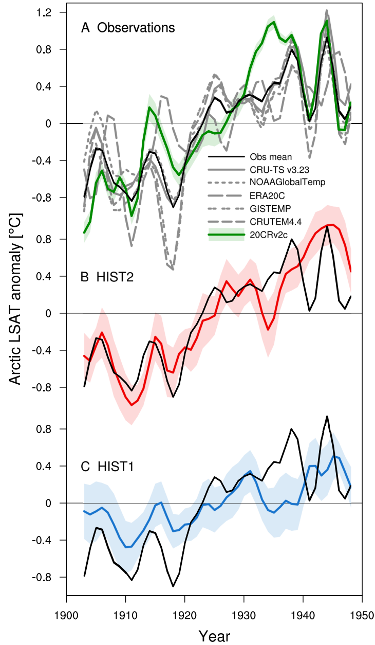
Fig. 2. Comparison of observed and simulated Arctic mean LSAT variations (60°-90°N). Time series of November-March mean Arctic LSAT anomaly, based on (A) observations, (B) HIST2, and (C) HIST1 experiments. For observations, six datasets are obtained from CRU-TS v3.23 (36) (gray solid line), NOAA GlobalTemp (33) (gray dotted line), ERA-20C (28) (gray long-dashed line), GISTEMP (34) (gray double-dotted line), CRUTEM4.4 (35) (gray short dashed line), and 20CRv2c (37) (green line with shading). The observational mean is superimposed in black. Shading indicates the two-tailed 95% confidence interval for each ensemble mean. All time series are smoothed with a binomially weighted 5-year running average.
