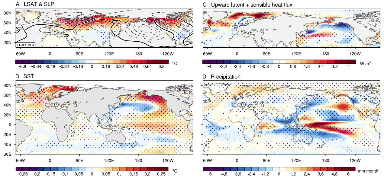
Fig. 4. Composite anomalies regressed onto the normalized Arctic mean LSAT anomaly, based on 37 CMIP5 piControl simulations. (A) LSAT (shading; ^{\circ}\text{C} ) and SLP (contour interval 0.15 hPa, zero contours thickened, positive solid, and negative dashed), (B) SST ( ^{\circ}\text{C} ), (C) upward latent and sensible heat fluxes ( \text{W m}^{-2} ), and (D) precipitation ( \text{mm month}^{-1} ). Stippling indicates the composite regression anomalies exceeding the 95% confidence level.
