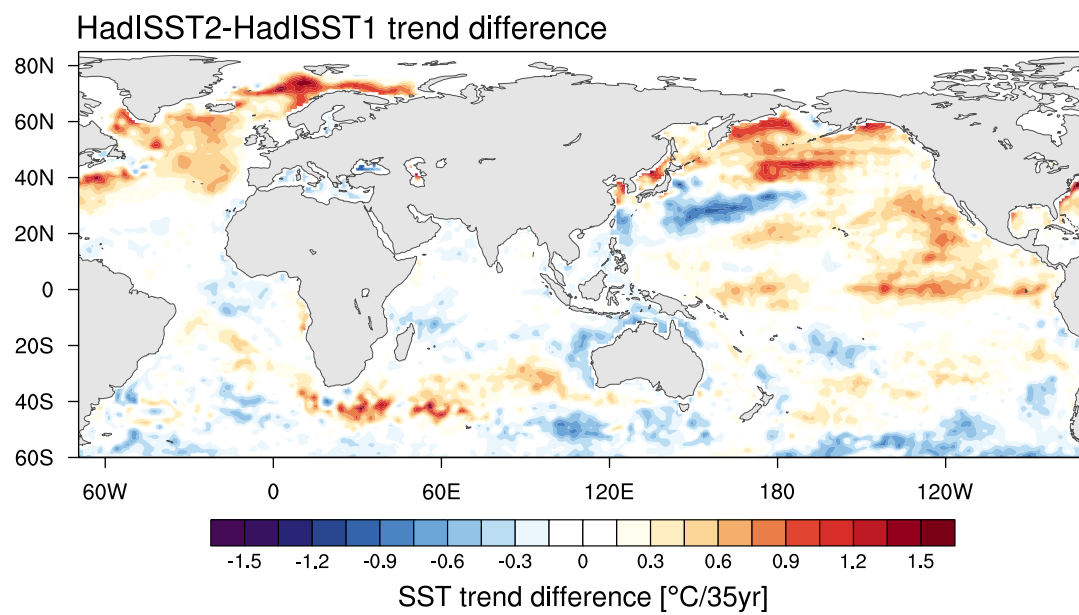
Fig. S2. SST trend difference between HadISST2 and HadISST1 for 1908-1942.
