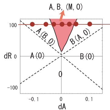
Figure 5. Stability diagram of the equilibrium solution to (3.9) for \delta = 0.1 . The dashed lines show neutral curves. A, B, M , and 0 without parentheses denote stable solutions and those with parentheses denote unstable solutions. The A-mode and B-mode are stable simultaneously in the grey region. We investigate (5.1) for the points (dA, dR) shown by dots.
