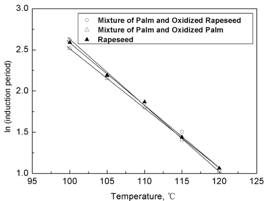
Fig. 6. Logarithm of induction period as a function of temperature for various biodiesel and mixtures of biodiesels, in order to get biodiesel that has the same induction period at 110^{\circ}\text{C} , the prepared palm and rapeseed biodiesels were stored at 50^{\circ}\text{C} for 72 and 36h to decrease their induction periods and mixed the oxidized biodiesels with newly prepared palm biodiesels.
