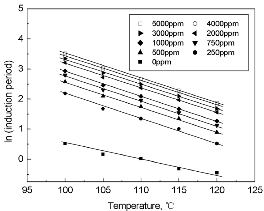
Fig. 4. Logarithm of induction period as a function of temperature for safflower biodiesel stabilized with various concentration of propyl gallate.
