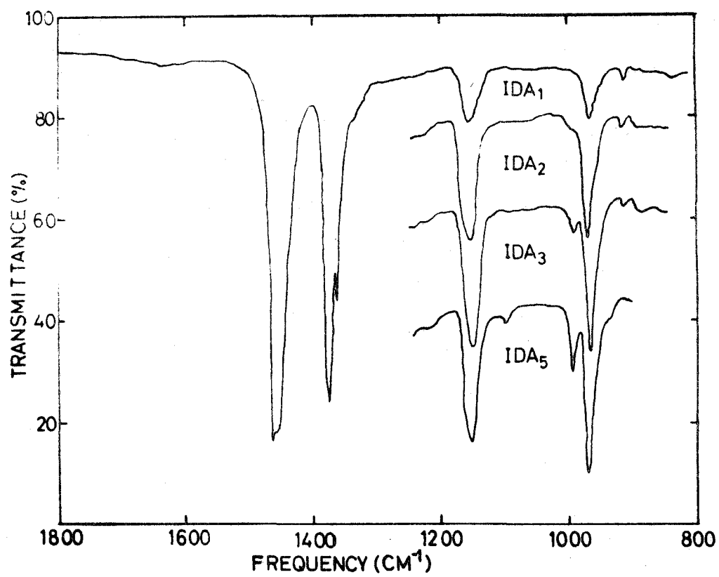
Fig. 5-4 IR-spectra of low-molecular-weight, isotactic polypropylene after hydrogenation.
