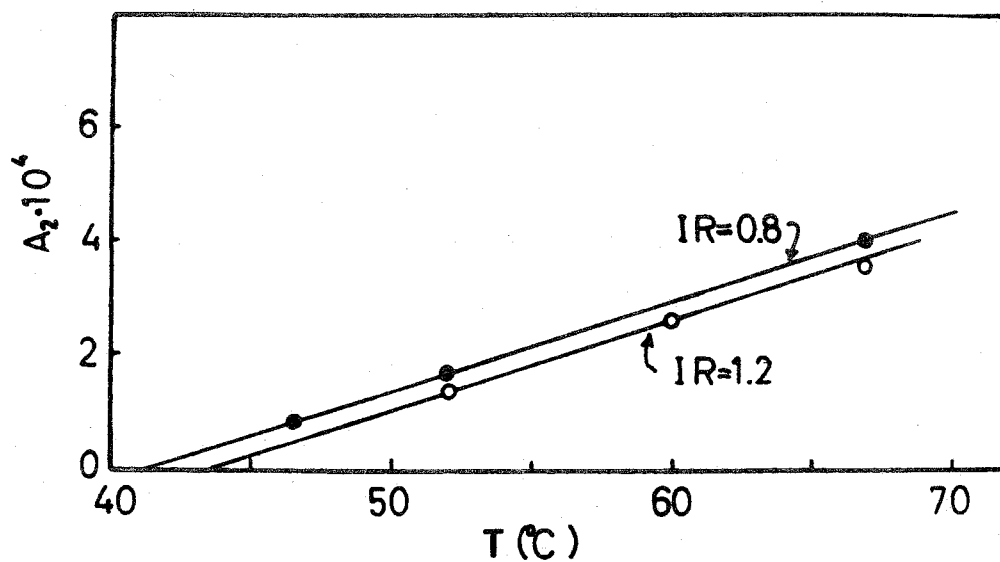
Fig. 3-3 Temperature dependences of A_2 for SP-T 5 and SP-HE 234 studied by light scattering. The approximate estimates of theta temperatures are 41 ^{\circ} and 43.5 ^{\circ} C for the former and latter sample, respectively.
