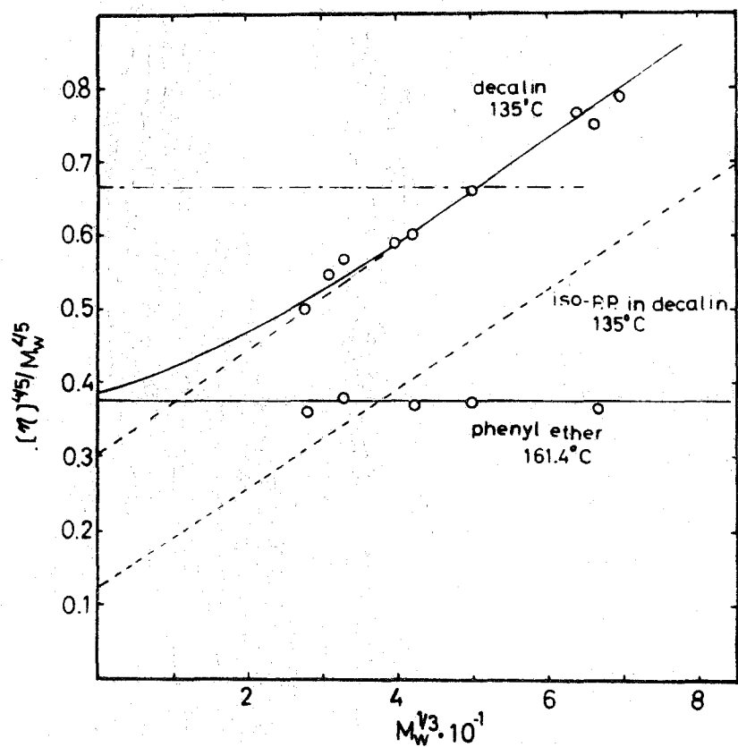
Fig. 3-12 Plots of eq.(13) with [\eta] - M_w relationships obtained by Chiang for polyethylene in decalin and phenyl ether (●-solvent). The same plot for isotactic polypropylene in decalin at 135°C is given for comparison by dotted line.
