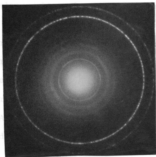
Fig. 4-3 A ring-form electron diffraction pattern observed from single crystal aggregates.
