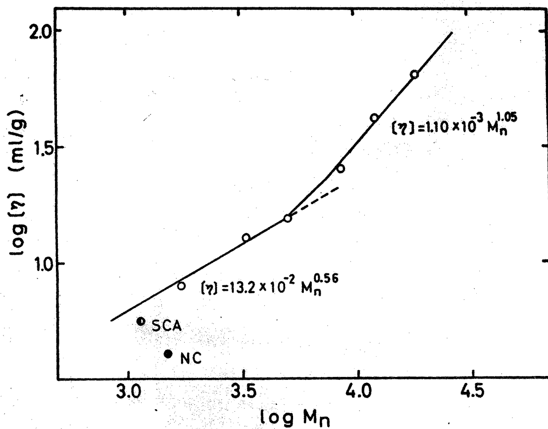
Fig. 5-9 Plots of \log[\eta] vs. \log M_n for SBP fractions \circ , NC \bullet , and SCA \bullet in cyclohexane at 30^\circ\text{C} .
