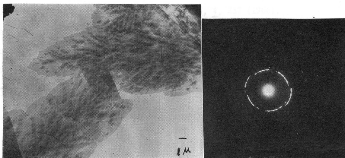
Fig. 4-5 Representative single crystals of poly- \epsilon -caprolacton grown from 2-ethoxyethanol solution and the correspond- ing electron diffraction patterns.
