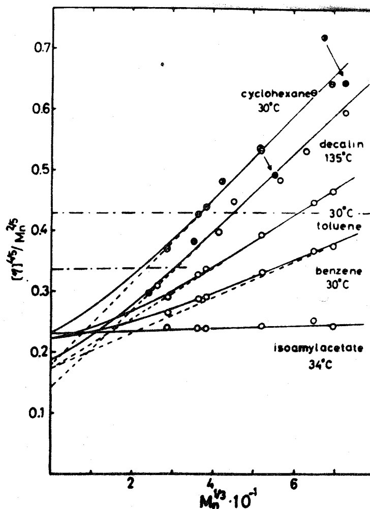
Fig. 3-4 Plots of eq.(13) with [\eta] - M_n relationship reported by various authors for atactic polypropylene in different solvents. The lower and upper chain lines indicate the limits of application of eq.(13) for the system in decalin at 135°C. and for the other solvent systems, respectively. For details, see Text.
