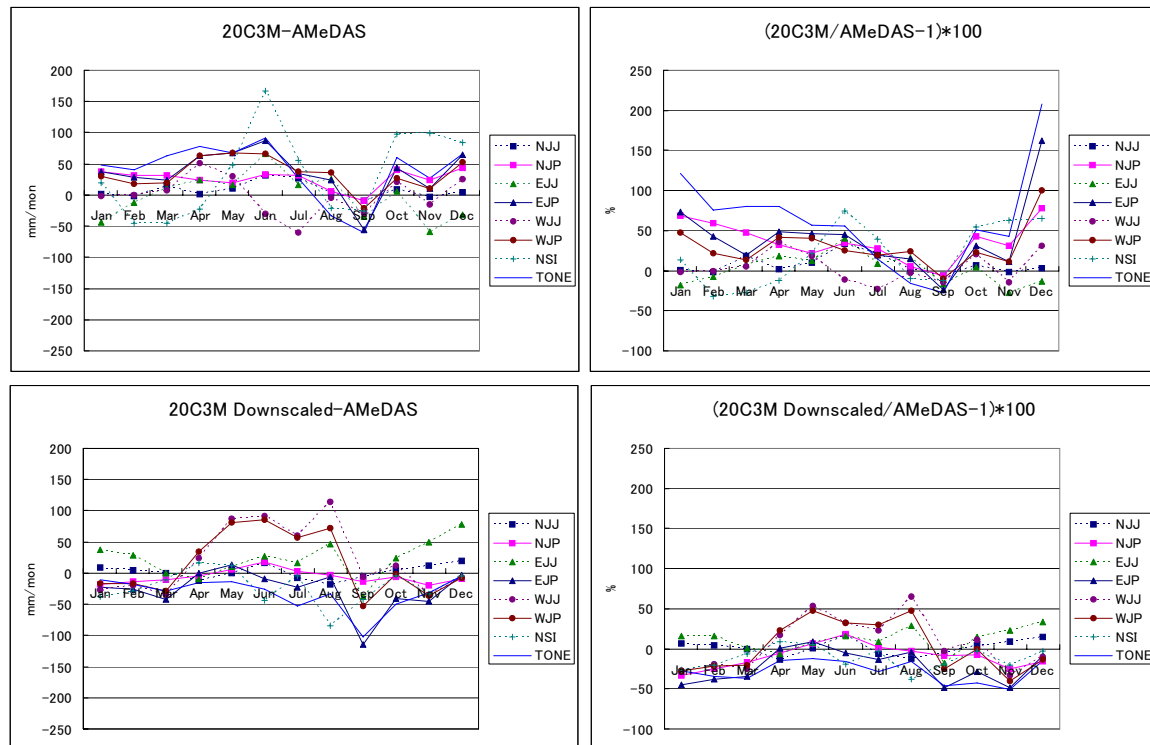
Fig.6 Errors in precipitation between the observations and the raw CGCM data (upper panels) and that between the observations and the downscaled results (lower panels). Left panels show raw differences (mm/mon) and right panels show ratios of difference (%). See Fig.5 for the line legends.
