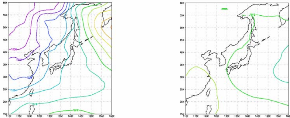
Fig. 4 SLP patterns of the clusters which have the largest number of members in January (left) and in August (right).
