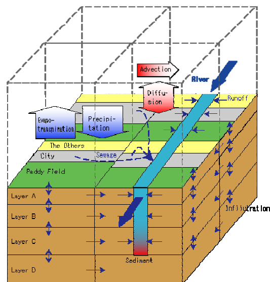
Fig. 2 The schematic of a kind of distributed runoff model generally known as Hydro-BEAM; The watershed is modeled as a uniform array of multi-layered mesh cells, each containing information regarding surface land use characteristics, ground surface slope and runoff direction, and the presence/absence of a channel.
