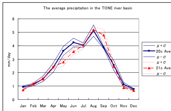
Fig. 8 The average precipitation in the Tone River basin; Solid blue and dashed red line shows the result of the 20th and the 21st century, respectively. Thin lines show the values added/subtracted one standard deviation to/from the average.
