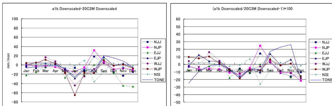
Fig.7 Same as Fig.6 but for differences between the downscaled result of the 20th century and the result of the 21st century; See Fig.5 for the line legends.
