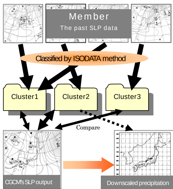
Fig. 1 The schematic of the downscaling technique presented here. See text for detail.
