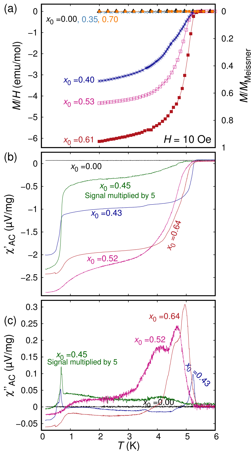
Figure 5. (a) DC magnetization as a function of temperature of \text{Sr}_{3-x}\text{SnO} samples prepared with various values of x_0 . Superconductivity appears for x_0 > 0.35 and becomes much weaker for x_0 \geq 0.7 . (b) Real and (c) imaginary parts of AC susceptibility, \chi_{AC} , normalized by the sample mass, plotted as functions of temperature. Two superconducting transitions at 5 K and 1 K appear for superconducting samples.
