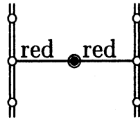
Figure 1: A configuration tree
