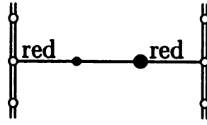
Figure 3: A configuration tree of \exp z^2
