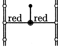
Figure 4: A configuration tree of a decorated \text{Cerf}(z)
