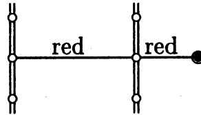
Figure 1: A configuration tree
