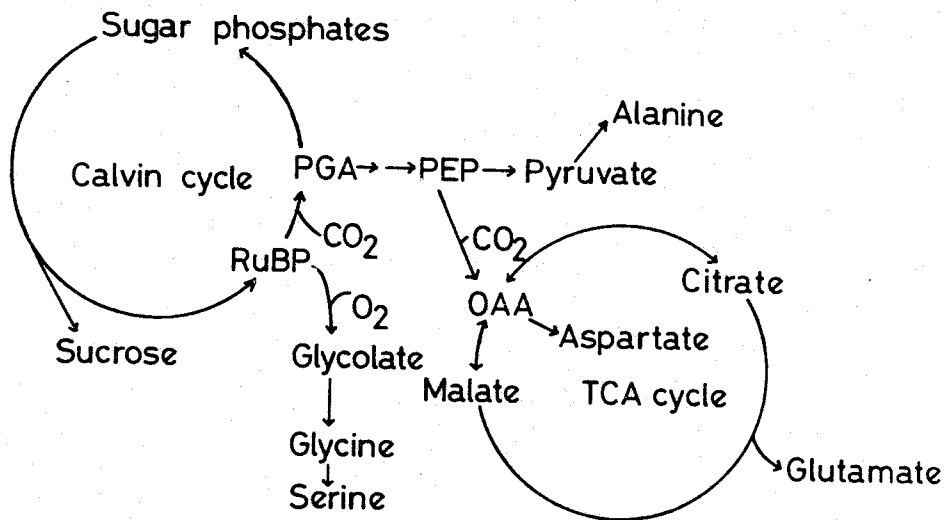
Fig. 19. CO 2 fixation and the related metabolic pathway
