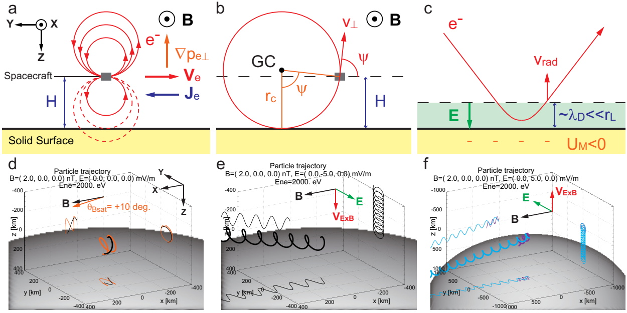
Figure 1. Schematic illustration of (a) the gyro-loss effect and the diamagnetic current, (b) the critical gyroradius, r_c , gyrophase, \psi , perpendicular velocity, v_\perp , spacecraft orbital height, H , and the guiding center of the electron, GC, and (c) an electron trajectory near the negatively charged lunar surface; \mathbf{v}_{rad} is the radial velocity component to the Moon, and the electric field \mathbf{E} produced by the negative surface electrostatic potential U_M is shielded within a few Debye lengths, \lambda_D , which is much smaller than the electron gyroradius, r_L . Sample electron trajectories (d) obtained from reverse tracking calculations, launched from a spacecraft altitude of 100 km with an energy of 2 keV, for a uniform magnetic field of 2 nT and no electric field; the black trace shows the trajectory for \theta_{Bsat} = 0^\circ and the orange trace shows that for \theta_{Bsat} = +10^\circ , (e) in the presence of a uniform electric field of E_y = -5 mV/m and (f) for E_y = 5 mV/m; the light blue trace shows the trajectory launched with an initial azimuthal angle of 250^\circ and an elevation angle of 0^\circ , the purple trace shows the trajectory with an azimuthal angle of 260^\circ and an elevation angle of 0^\circ .
