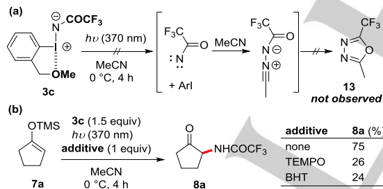
Scheme 4: (a) Exclusion of an acynitrile as an intermediate (b) Effect of radical scavengers.
