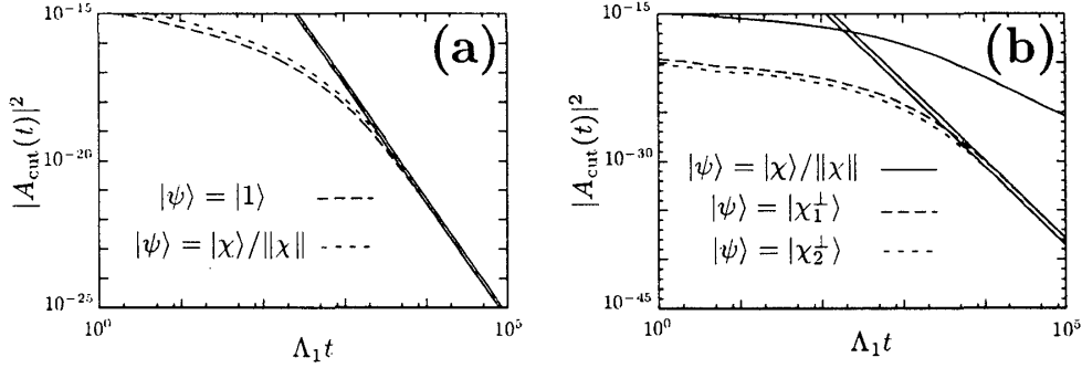
Figure 1: (a) |A_{\text{cut}}(t)|^2 for the initial states |\psi\rangle = |1\rangle and |\chi\rangle/\|\chi\| , and their corresponding asymptotes predicted by Eq. (3) (solid lines). (b) |A_{\text{cut}}(t)|^2 for the initial states |\psi\rangle = |\chi\rangle/\|\chi\| , |\chi_1^\perp\rangle , and |\chi_2^\perp\rangle . For comparison, two straight lines parallel to t^{-8} (solid lines) are also depicted.
