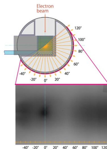
Fig. 1. Placement of a large Al activation foil (upper) and the resulting transfer image
