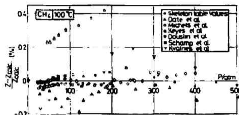
Fig. 2 Comparison of the calculated compressibility factor with the most probable values and with the experimental data along 100°C isotherm
