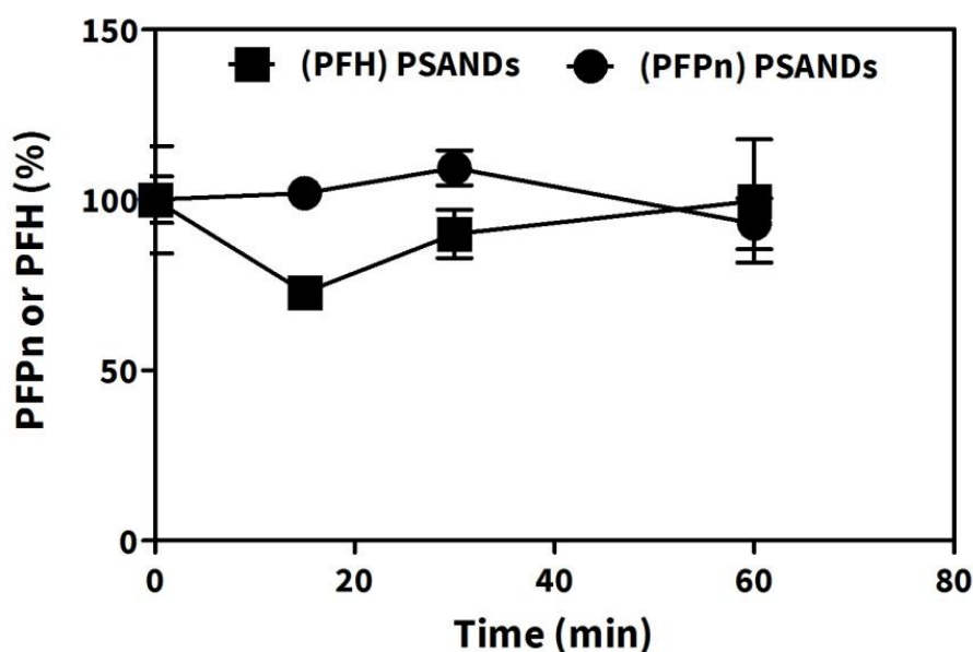
Fig. 12. In vitro PSAND's stability at 37 °C. Both PFPn and PFH nanodroplets were incubated in PBS at 37 °C, and samples at specific time points were collected for gas chromatography (GC-MS) analysis of PFPn and PFH. n = 3; mean \pm SEM
