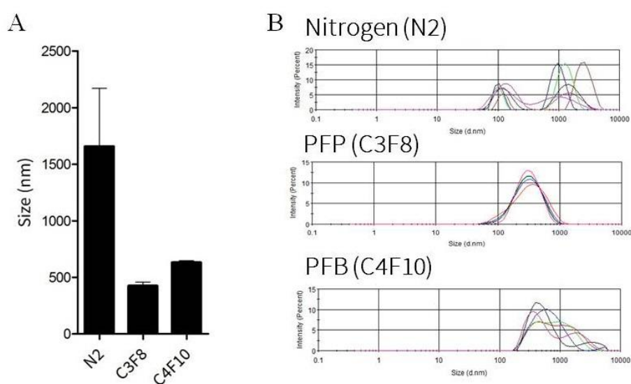
Fig.1. Size measurements of MFBs with different gases where C 3 F 8 is perfluoropropane gas, C 4 F 10 is perfluorobutane gas, and N 2 is nitrogen gas. (A) Mean bubble size (n = 3; mean \pm SEM). (B) Size
