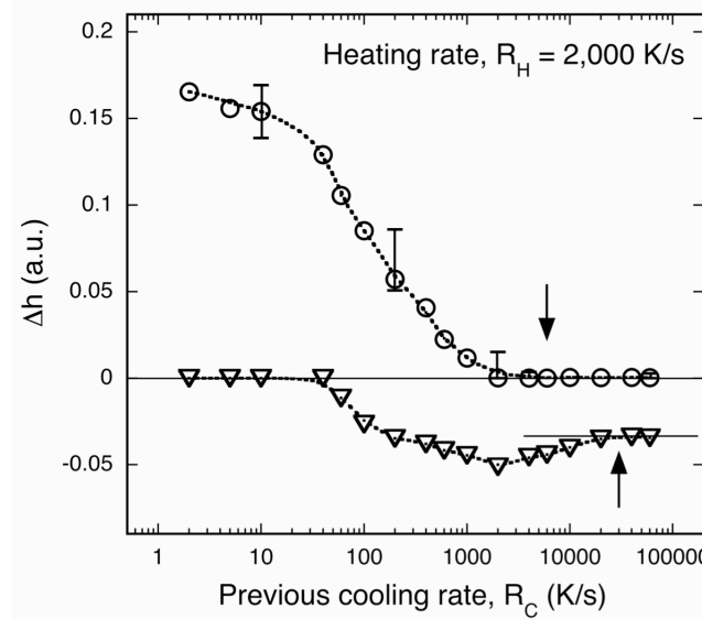
Fig. 6. Net enthalpy (upper panel) and exothermic enthalpy (lower panel) as a function of the previous cooling rate for the case of a heating rate R_H = 2,000 K/s.
