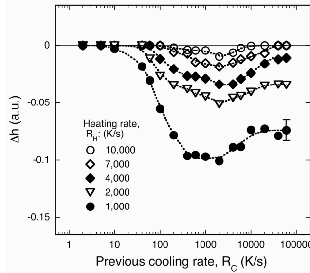
Fig. 7. Exothermic enthalpy as a function of the previous cooling rate for the different rates of heating.
