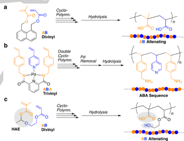
Scheme 1. Cyclopolymerizations to control alternating sequence. (a) Cyclopolymerization of AB-type divinylmonomer with cleavable spacer into two –COOH pendants, (b) doublecyclopolymerization of ABA-type trivinylmonomer on palladium complex, (c) cyclopolymerization of AB-type divinylmonomer with HAE spacer (this work).
